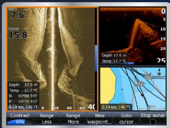
TrackBack™: Scroll back simultaneously through sonar history and chartplotter trail from sonar or StructureScan™ display to easily mark waypoints, and continue to record data while reviewing history.
